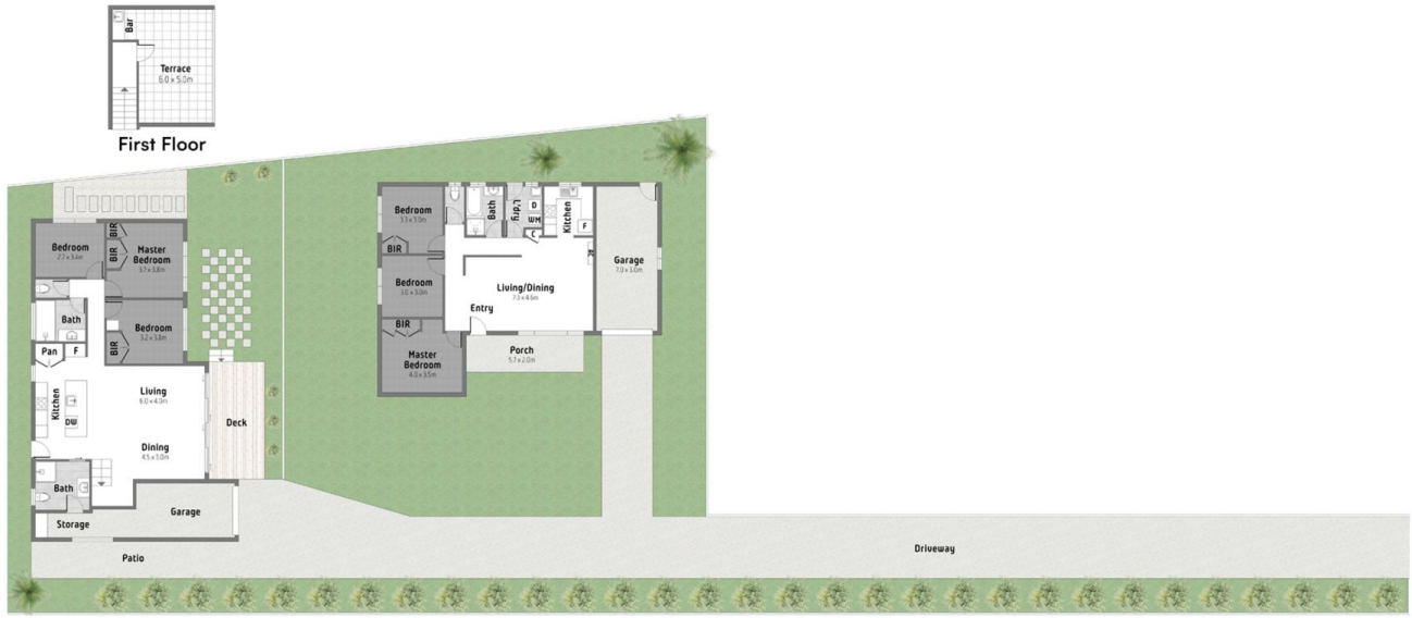
Ground Floor and Site Plan
